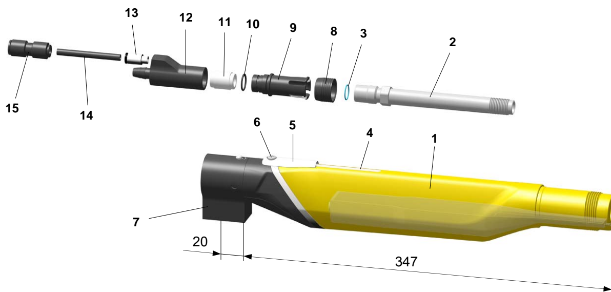
OptiGun GA03-P – gun body
