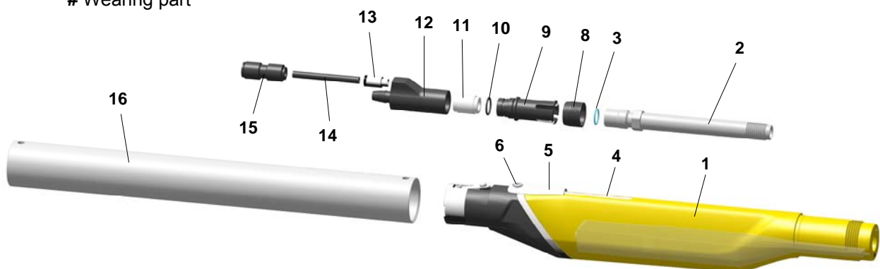
OptiGun GA03-P-X – gun body
