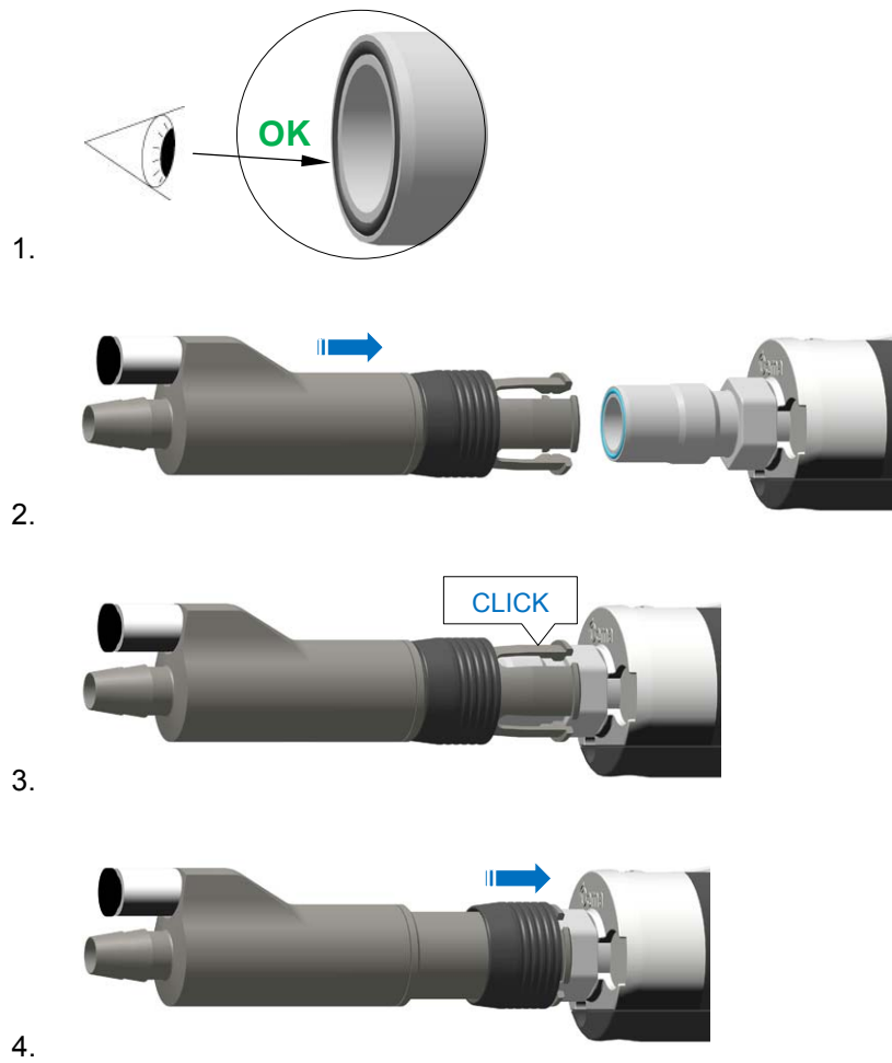
Connecting the diffuser
