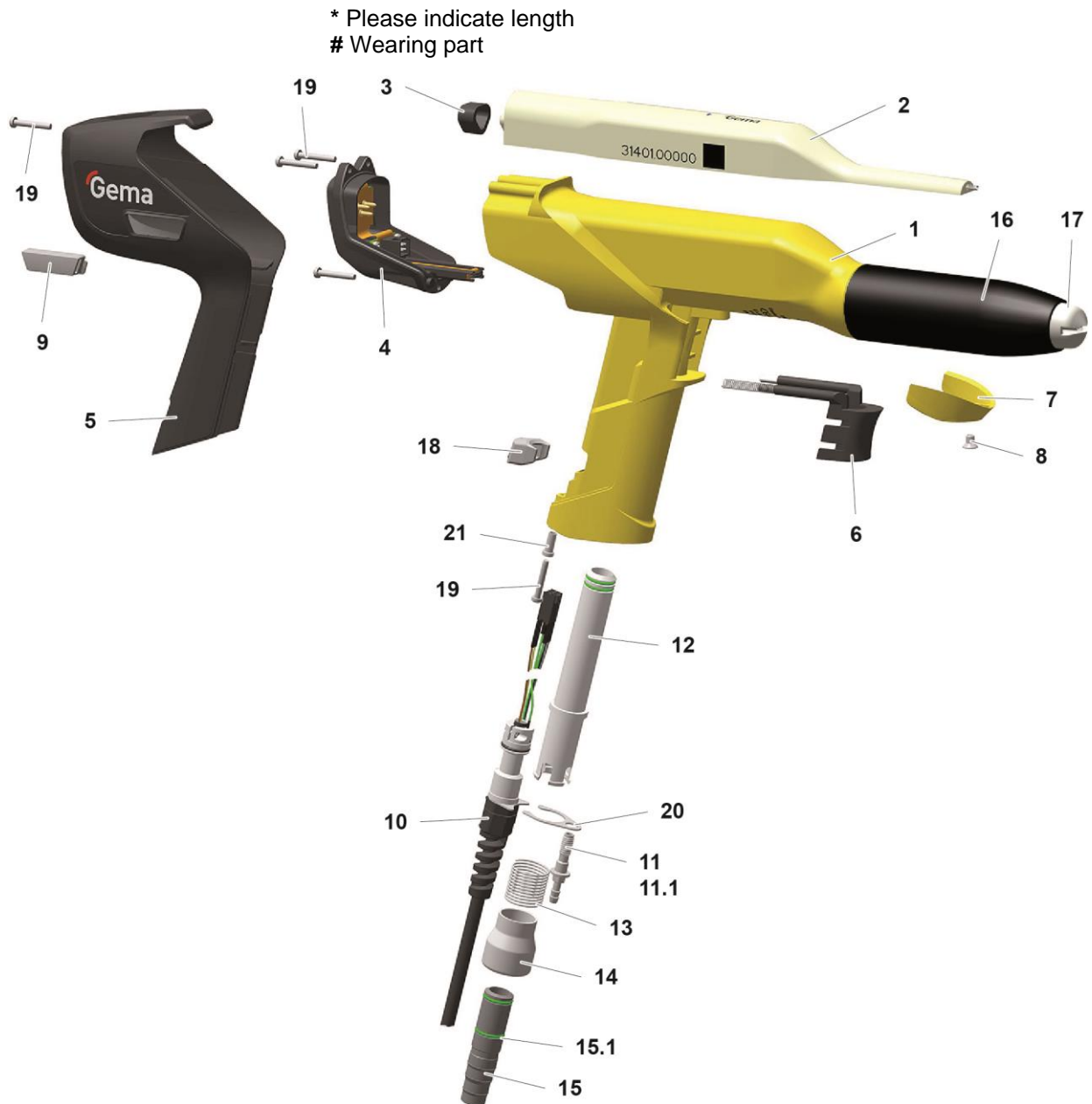
fig. 10: OptiSelect Pro GM04 – spare parts
